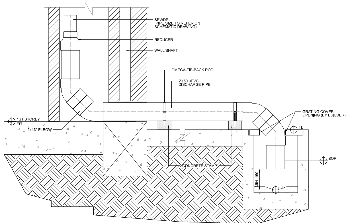
TYPE 2 TYPICAL DISCHARGE DETAIL
