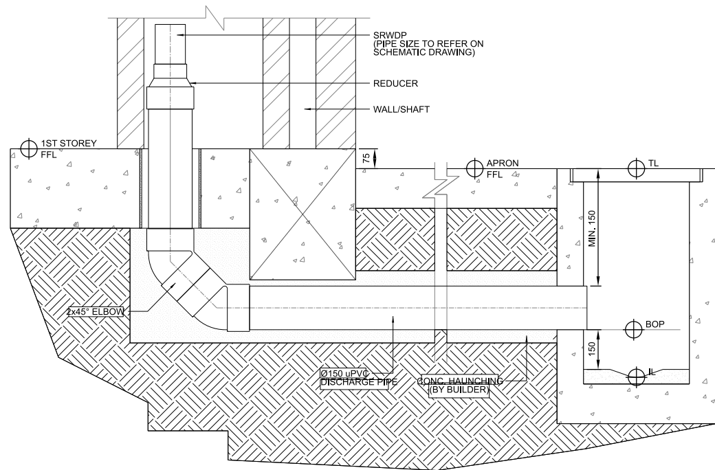
TYPE 1 TYPICAL DISCHARGE DETAIL
